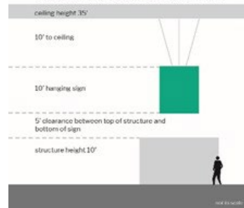
Structure at a max height of 10' Sign at a max height of 10'
